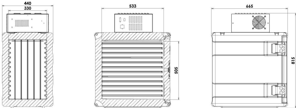
Model with cooling unit on top static K90AFTSDYM0 and K90AFTSDZM0
