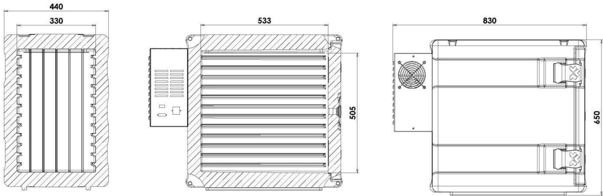
Model with cooling unit on back static K90AFDSDYM0 and K90AFDSDZM0
